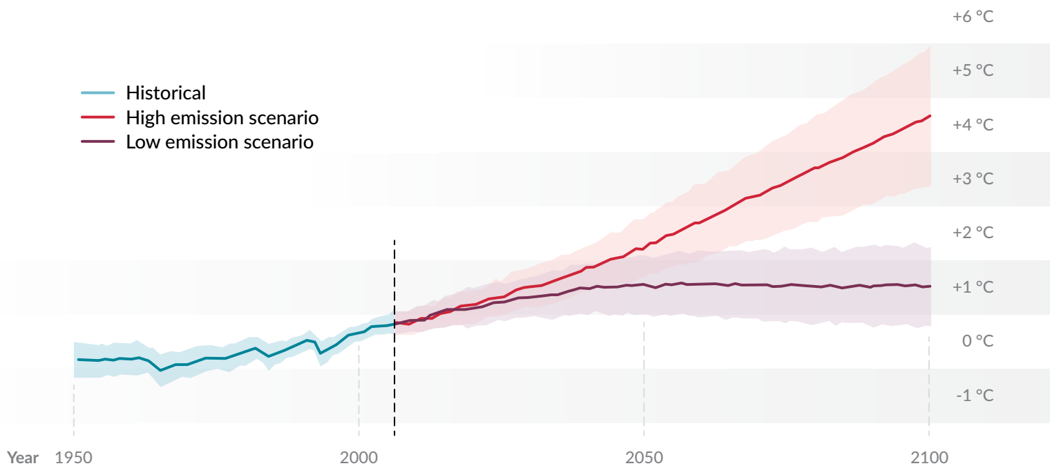
Figure 4: Projections for global average surface temperature change (Source: Fifth Assessment Report of the Intergovernmental Panel on Climate Change)
